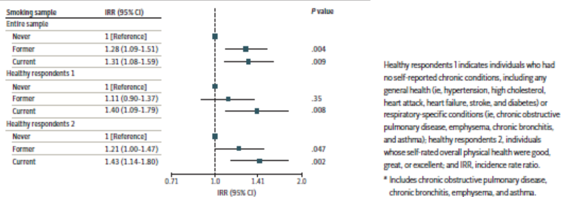
Figure. Associations of e-Cigarette Use With the Risk of Respiratory Disease a
